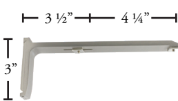
AVA223-XX Double Wall Bracket
