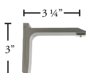
AVA221-XX Single Wall Bracket
