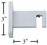
MON241-SS Single Wall Bracket
