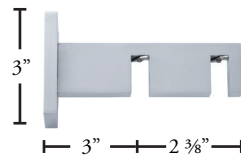
MON243-SS Double Wall Bracket
